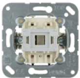
Switch insert (intermediate) 10 AX, 250 V ~ EP407U
