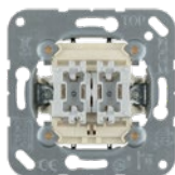
2-gang universal switch insert 10 AX, 250 V ~ EP409U
